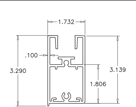
4 PANEL TOP RAIL
