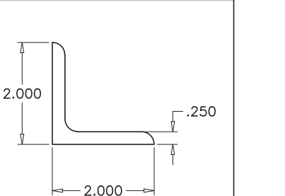
16 SILL ANGLE
