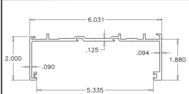
1 FRAME HEAD
