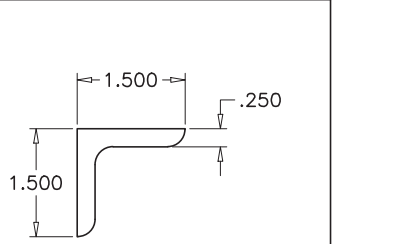
29 SHEAR CLIP
