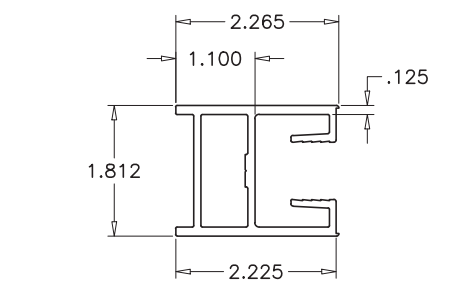
6 FIX. PANEL JAMB STILE
