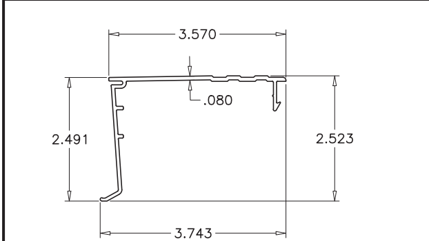
12 SILL THRESHOLD TRIM
