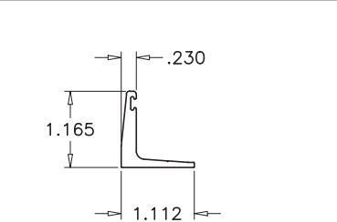
14 SILL ANTI-BLOWOUT CLIP
