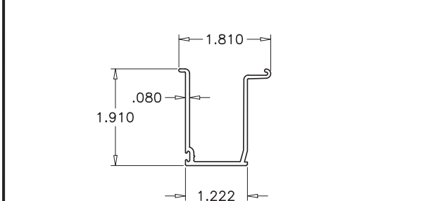
2 FRAME SILL
