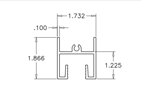
4 PANEL TOP RAIL
