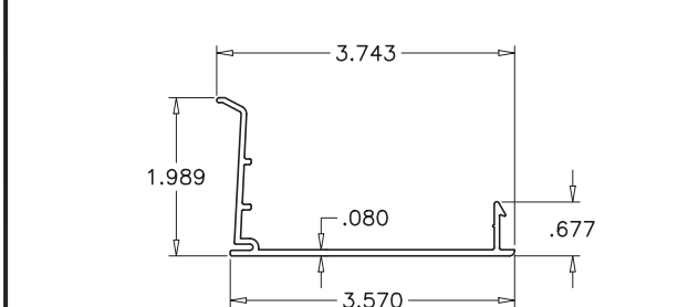
10 FIX. PANEL STOP
