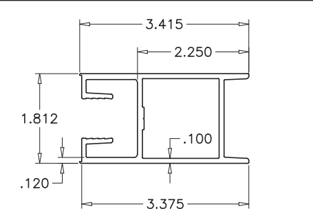
7 OPERATING PANEL JAMB STILE
